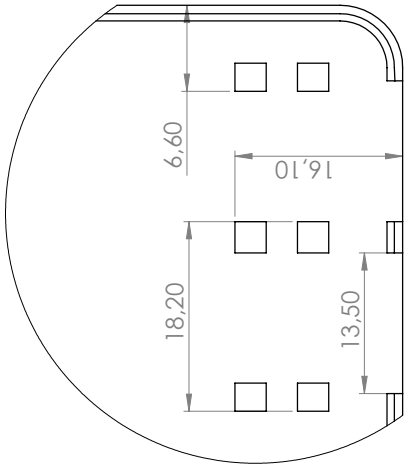
DETAIL F SCALE 2:1
